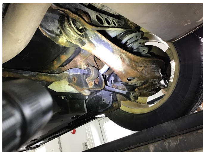
1.2 Rust bakstilling/travers
