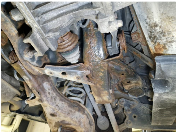
1.1 Rustdannelser bakre travers.
